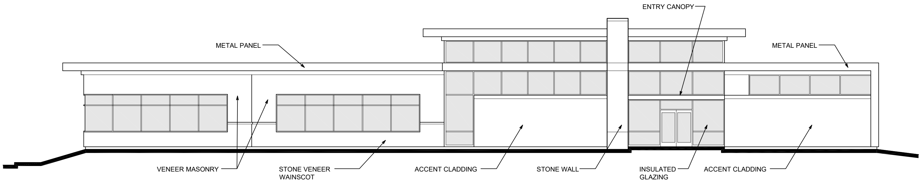
PRELIMINARY EAST ELEVATION
