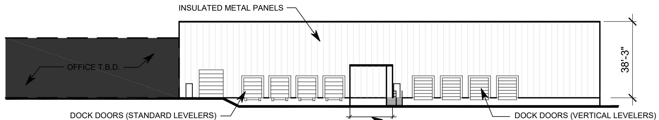
NORTH ELEVATION
