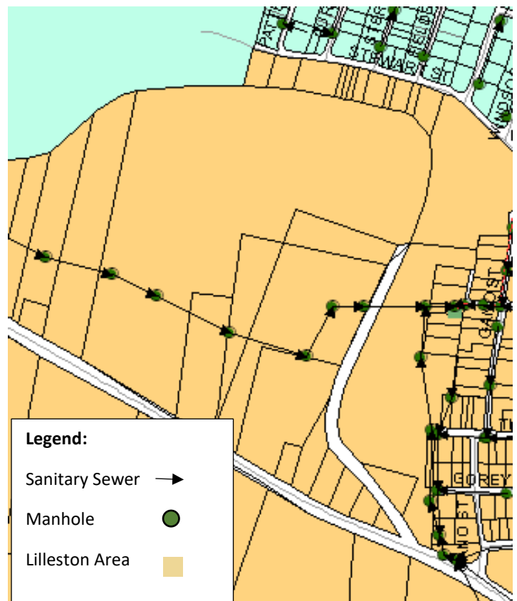
FIGURE 3: City of Paris Sanitary Sewer
